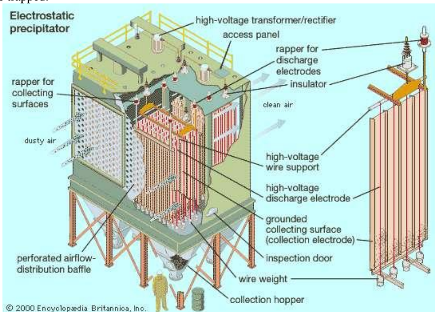
Figure 2: Electrostatic precipitator
